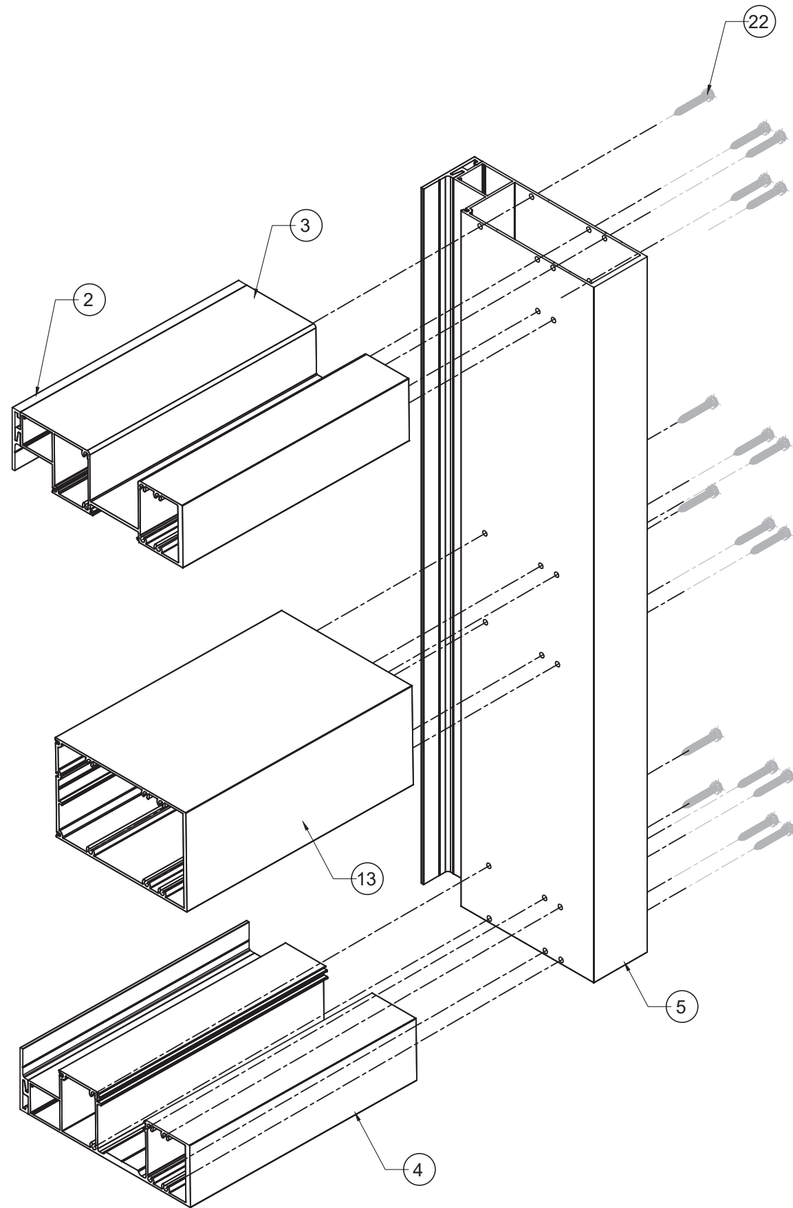
FRAME ASSEMBLY
